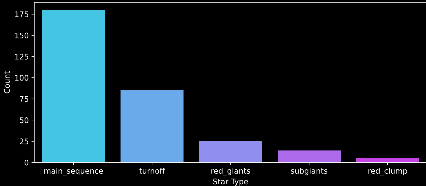
GALAH DR4 Field: [457] Count plot of Star Type
