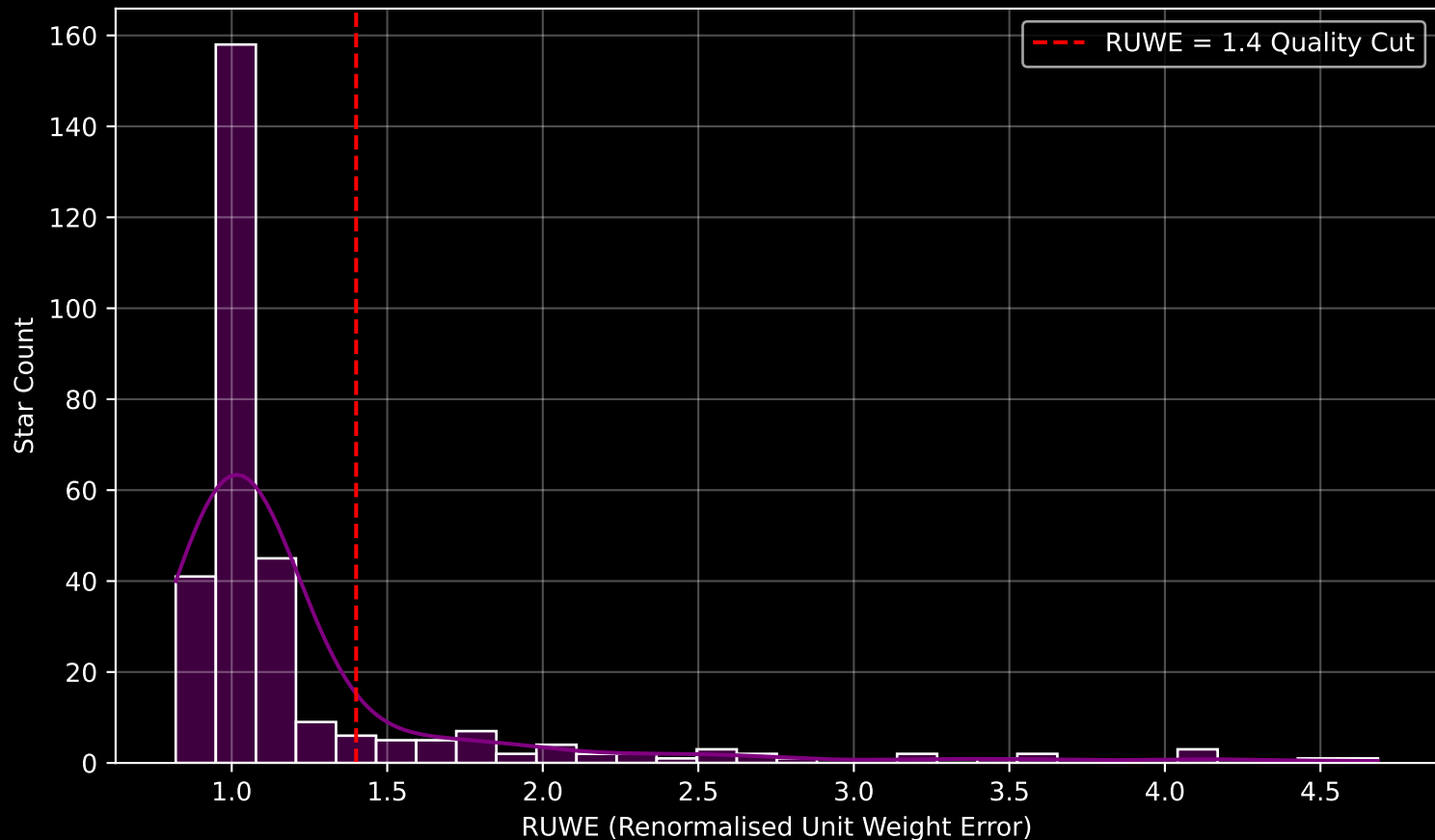
GALAH DR4 Field [457] RUWE Distribution (n= 303)
