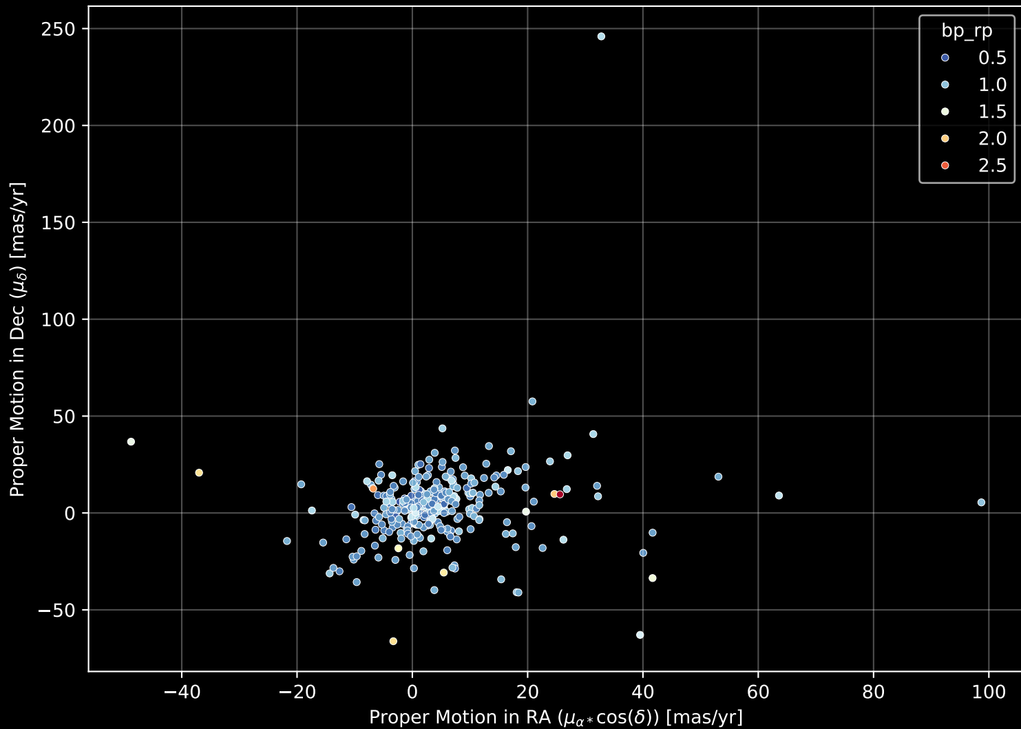
GALAH DR4 Field: [457] Proper Motion Diagram (n= 309)
